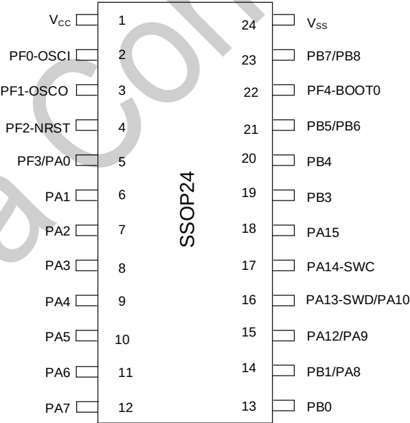
图 3-4 SSOP24 Pinout2 PY32F032E2xM7 (Top view)
