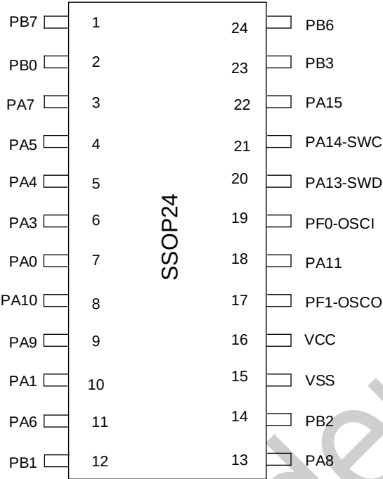
图 3-3 SSOP24 Pinout1 PY32F032E1xM7 (Top view)
